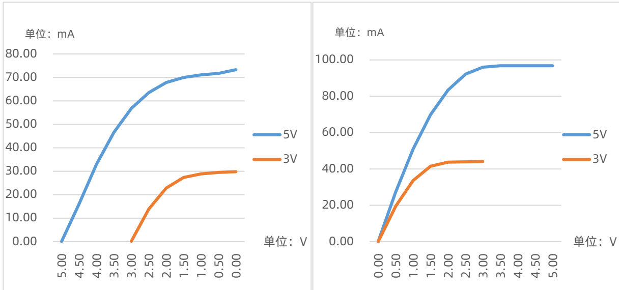
IOH 1 IOL 1
